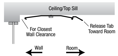
Flush Mount Option
